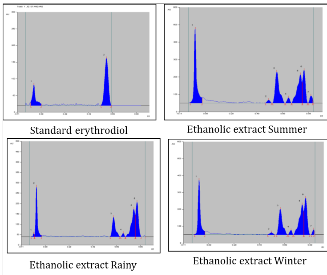
Figure 4 Densitogram of erythrodiol from A. scholaris
